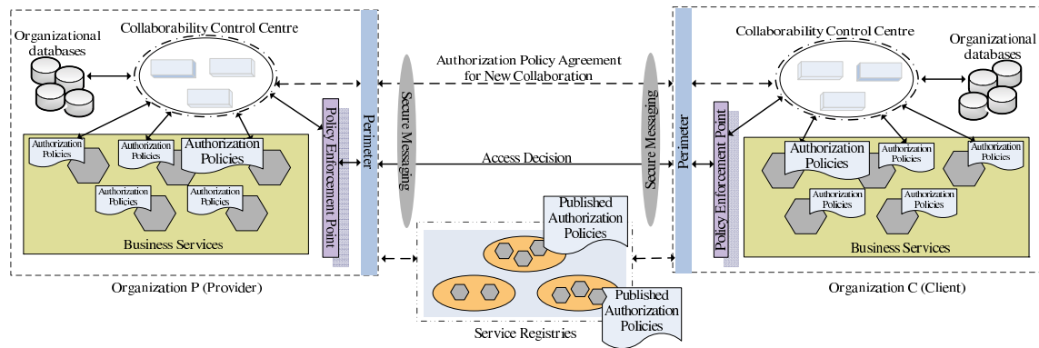
Figure 1: Policy Driven Authorization Control Framework
